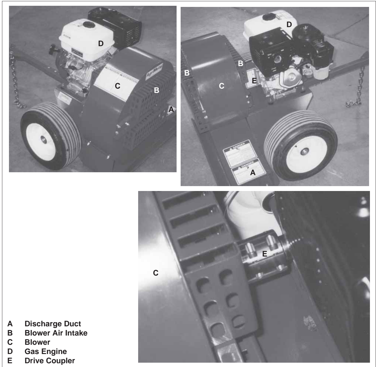
Fig. 4 PRINCIPLE COMPONENTS
