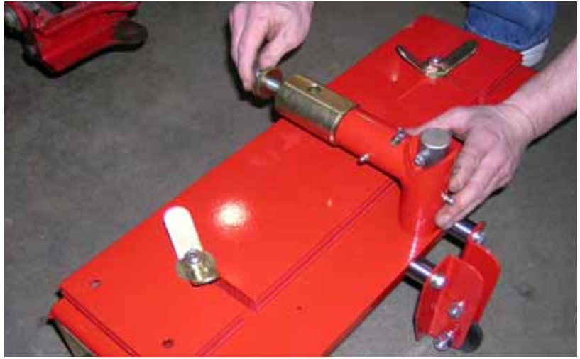
Fig. 6 MOUNTING FRAME ANCHOR BOLT (TORO MOD: 3200 SERIES)
