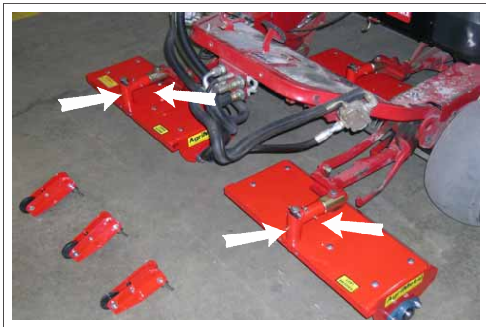
Fig. 19 HEAD ASSEMBLY (TYPICAL)
