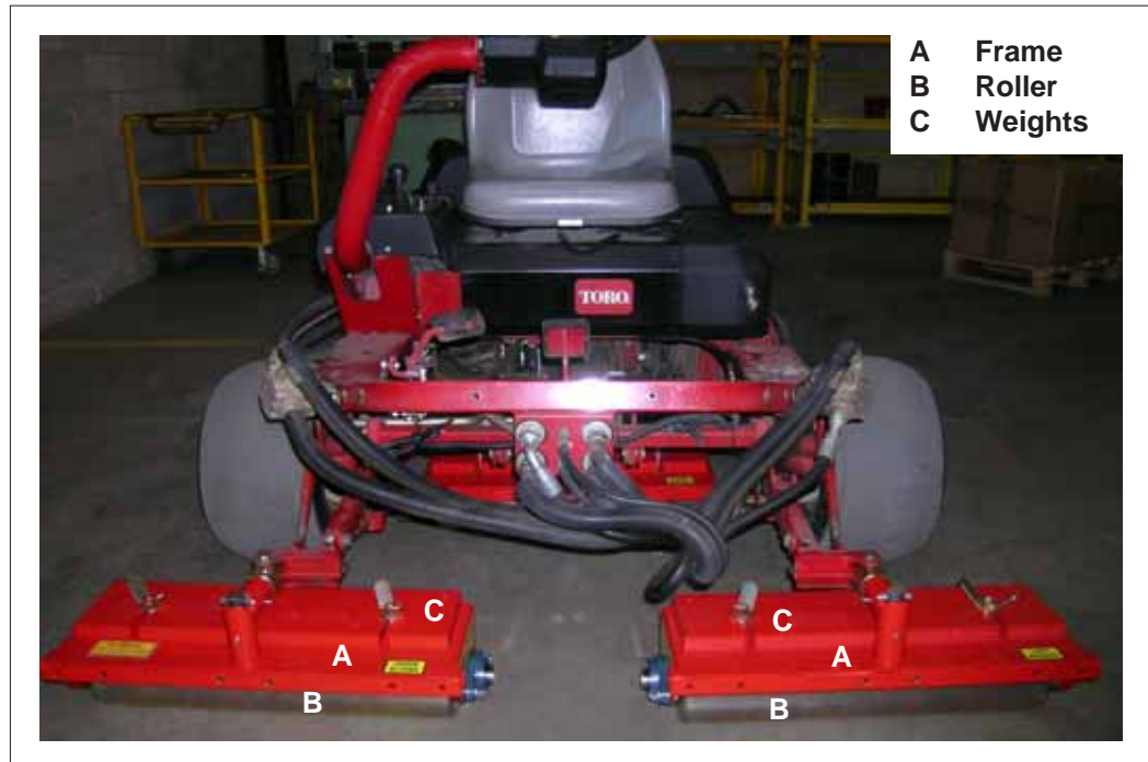
Fig. 12 PRINCIPLE COMPONENTS
