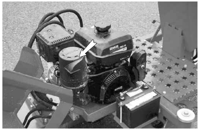
Fig. 31 AIR CLEANER
