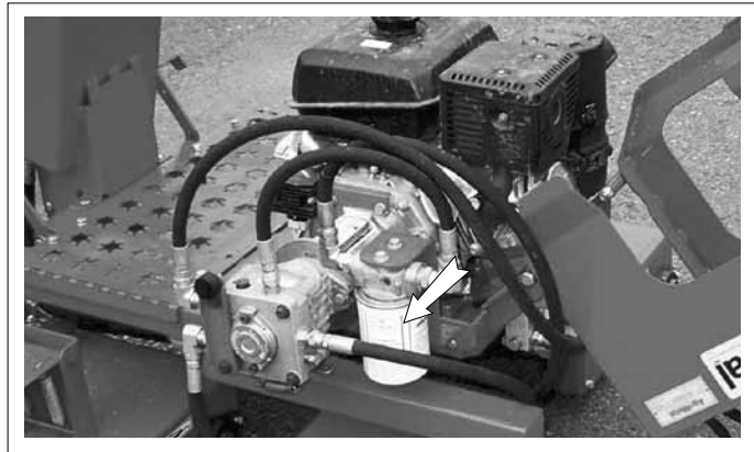
Fig. 34 HYDRAULIC FILTER
