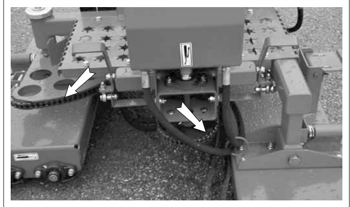
Fig. 37 STEERING ROLLER CHAIN
