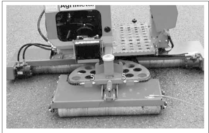
Fig. 42 ROLLER CHAIN ADJUSTERS (Typical)
