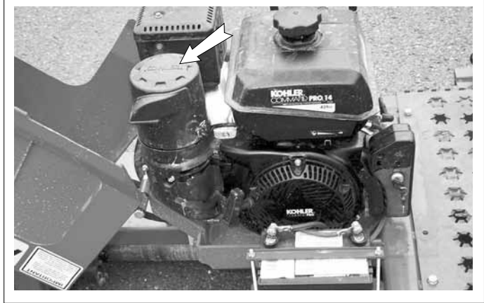
Fig. 39 AIR CLEANER
