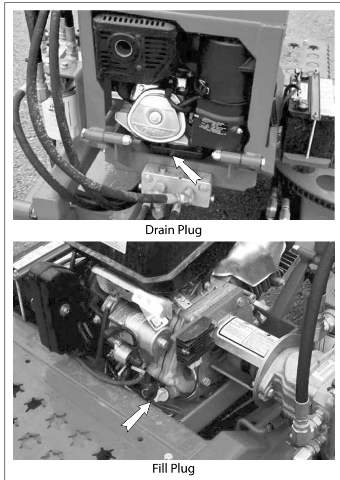
Fig. 40 ENGINE
