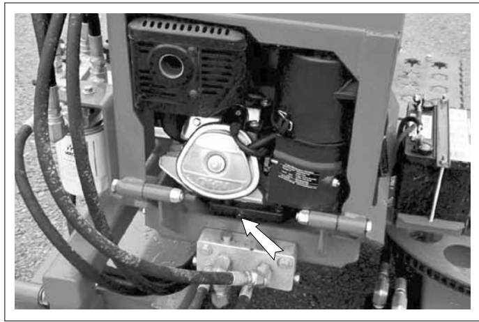
Fig. 32 DRAIN PLUG
