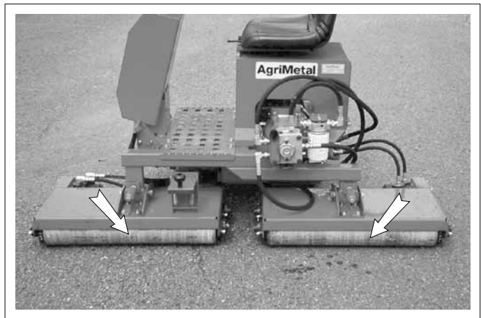
Fig. 27 ROLLER HEADS
