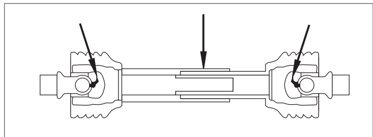
Fig. 26 PTO DRIVELINE
