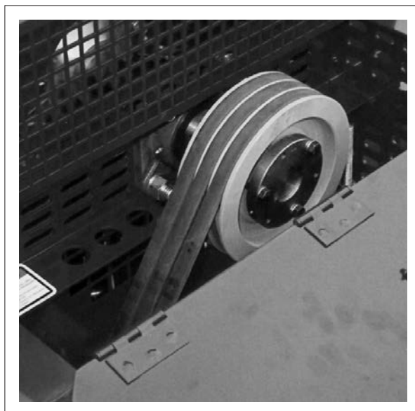
Fig. 31 DRIVE BELTS
