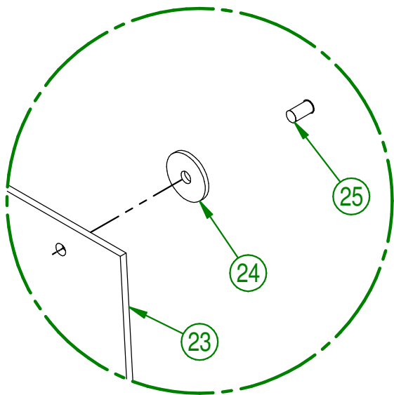
DETAIL D
