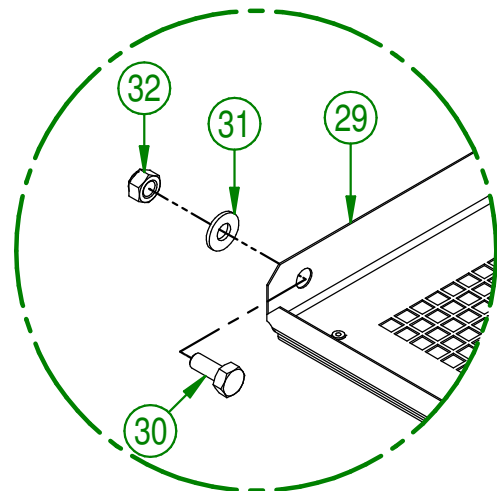
DETAIL E
