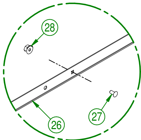
DETAIL F
