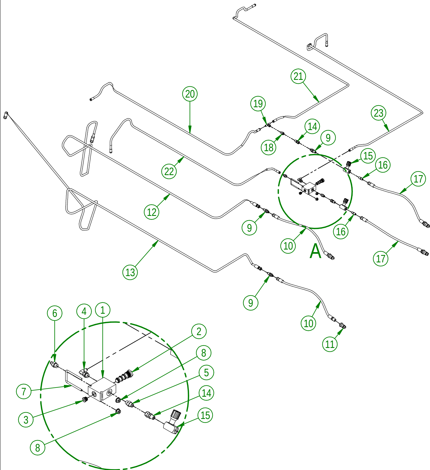
DETAIL A
